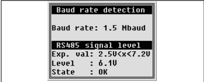
Figure 60: Baud rate detection
