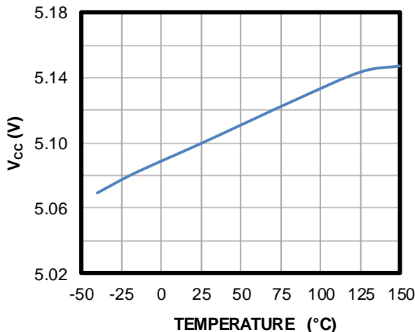
V_{CC} vs. Temperature V_{IN} = 12V
