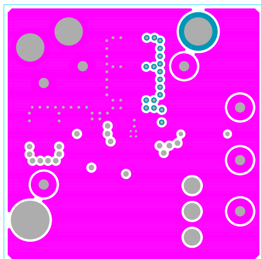
Figure 10. Layer 2
