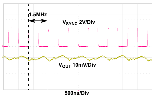
Figure 26. External Frequency Synchronization Waveform, V_{IN} = 3.3V , V_{OUT} = 1.2V , f_{SYNC} = 1.5MHz , I_{OUT} = 0A , C_{OUT} = 2 \times 22\mu F Ceramic
