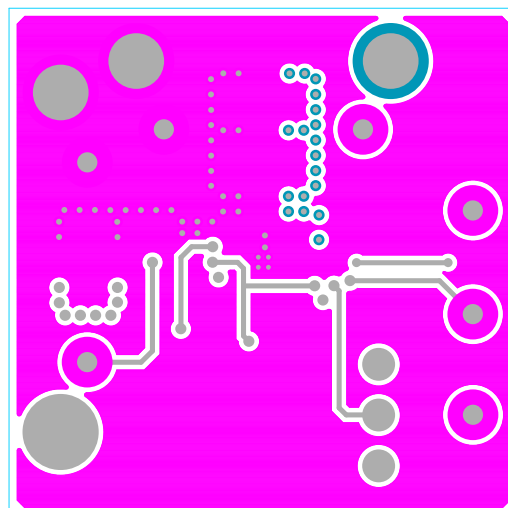
Figure 11. Layer 3
