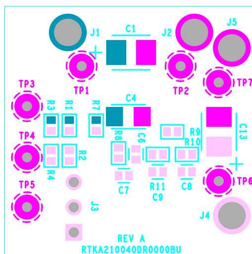
Figure 13. Silkscreen Bottom
