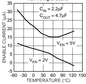
Enable Current Threshold vs. Temperature
