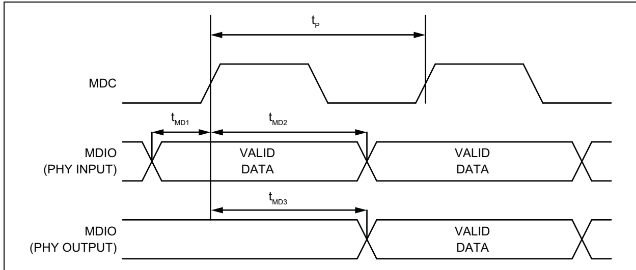
FIGURE 7-4: MDC/MDIO TIMING
