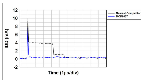
FIGURE 4-5: I_{DD} During Start-up.
