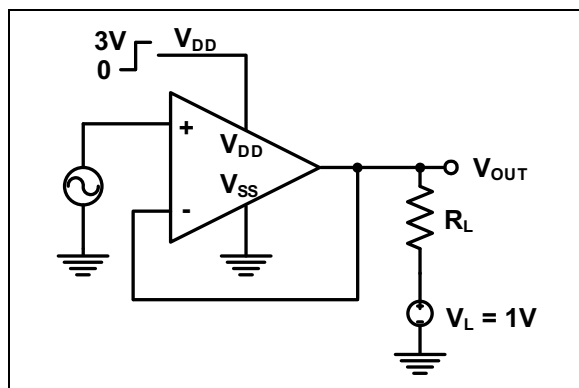
FIGURE 4-3: Start-up Test Circuit.
