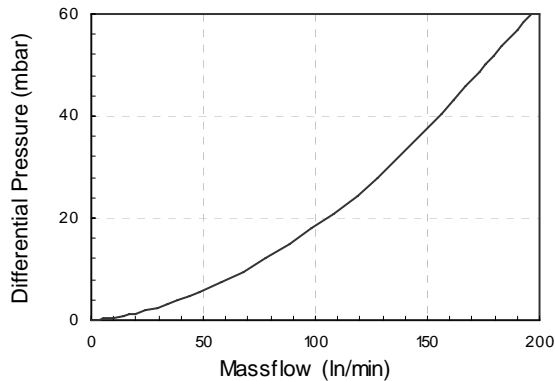
Figure 4: Differential Pressure vs. Mass Flow of CMOSens ® EM1 Device.
