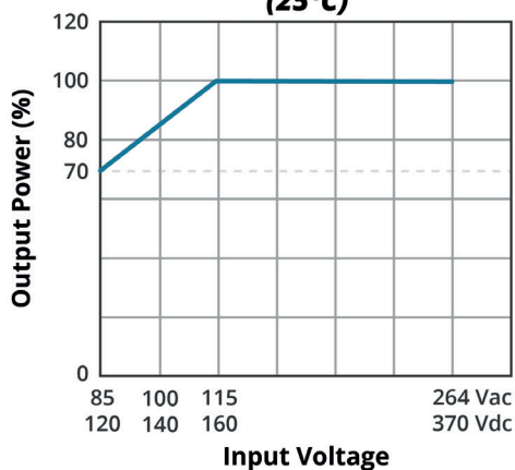
INPUT VOLTAGE DERATING CURVE (25°C)
