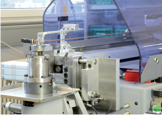
Automatic bending
