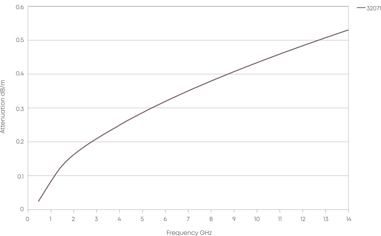
Attenuation (nominal values at +25 °C ambient temperature)
