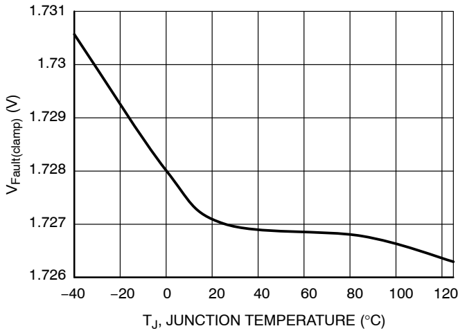
Figure 57. V_{\text{Fault}(\text{clamp})} vs. Temperature
