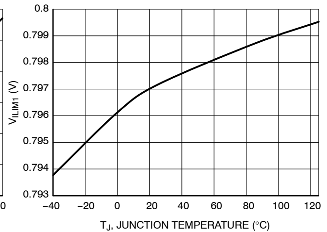
Figure 62. V_{\text{ILIM1}} vs. Temperature
