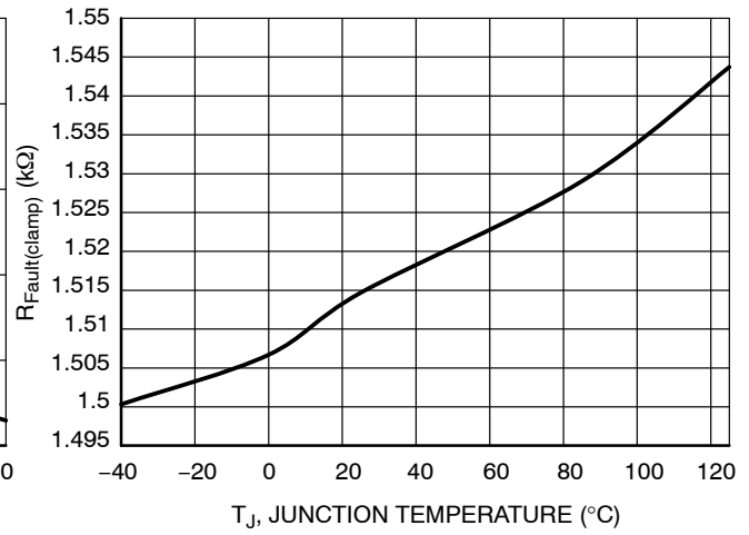
Figure 58. R_{\text{Fault}(\text{clamp})} vs. Temperature
