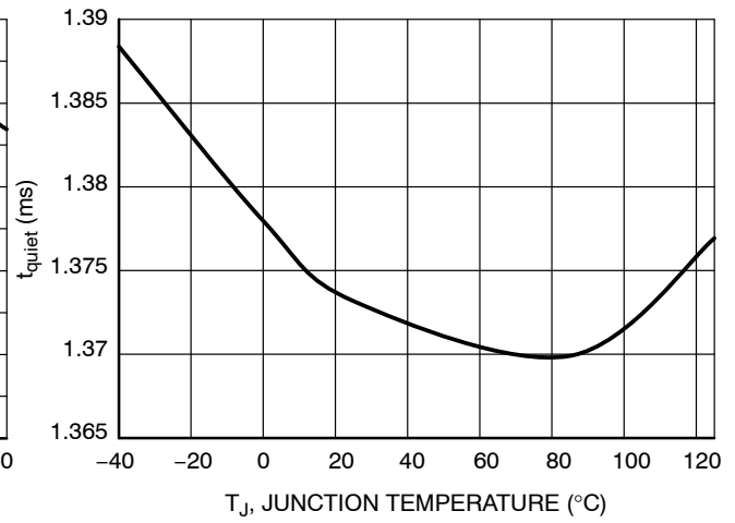
Figure 60. t_{\text{quiet}} vs. Temperature
