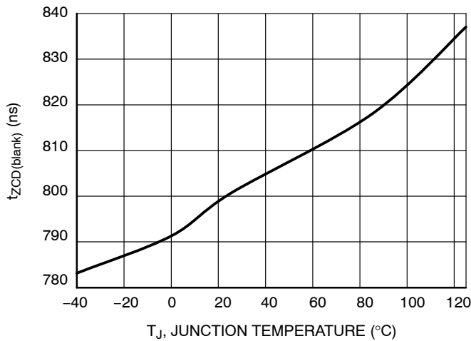
Figure 61. t_{\text{ZCD}(\text{blank})} vs. Temperature
