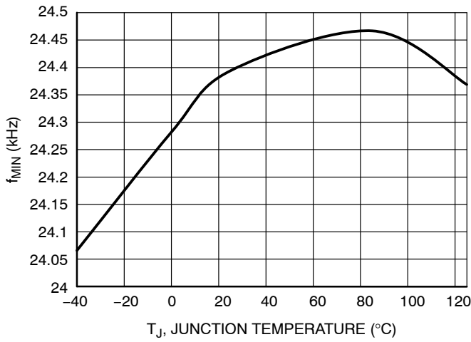
Figure 59. f_{\text{MIN}} vs. Temperature
