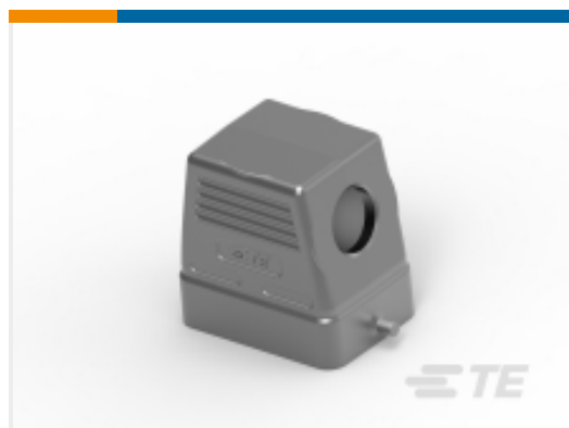
TE Part #T1310060121-000 H6B-TS-PG21
