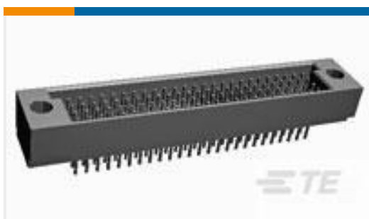
TE Part #532436-1 HDI PIN ASSY 4 ROW 100 POS
