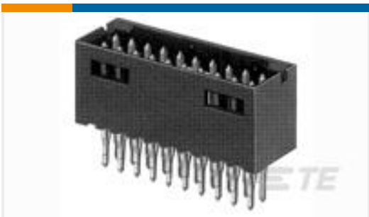
TE Part #5120823-1 Hard Metric Male Connector: Traditional Backplane, Mezzanine, 2mm
