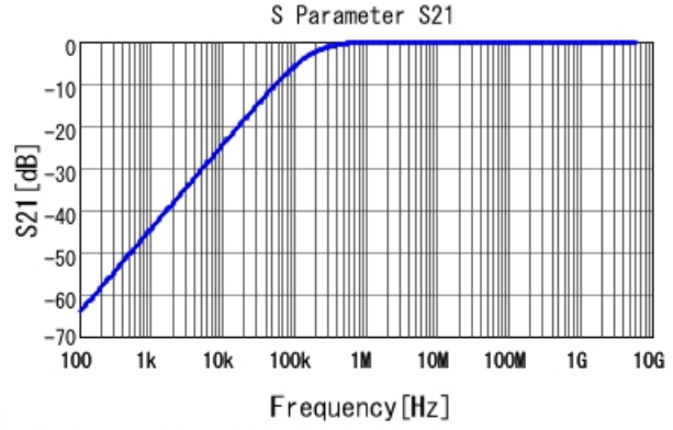
■ GRM033R71A103KA01 S21 DCOV, 25degC
