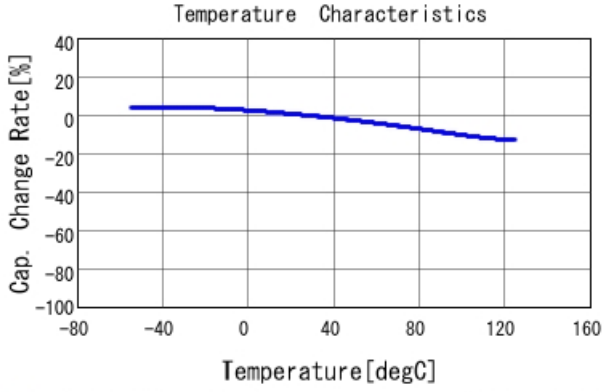
■ GRM033R71A103KA01 C-Temp. capchange, DCO. 0V, AC1. 0Vrm
