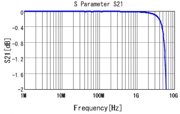
■ GRM31C5C1H563JA01 S21 DCOV, 25degC
