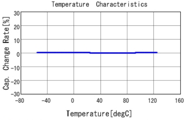
■ GRM31C5C1H563JA01 C-Temp. capchange, DCOV, AC1Vrms
