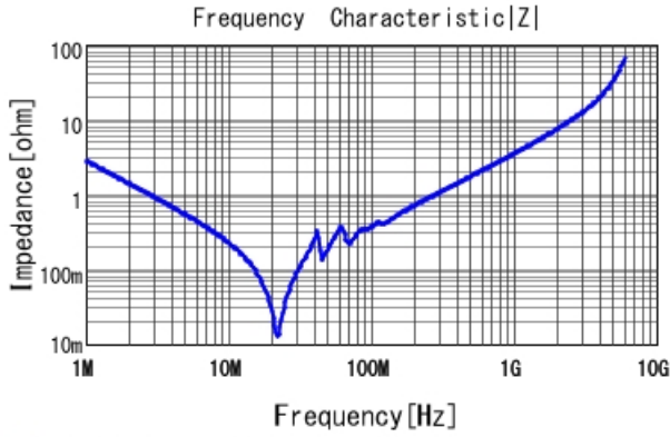
■ GRM31C5C1H563JA01 |Z| DCOV, 25degC
