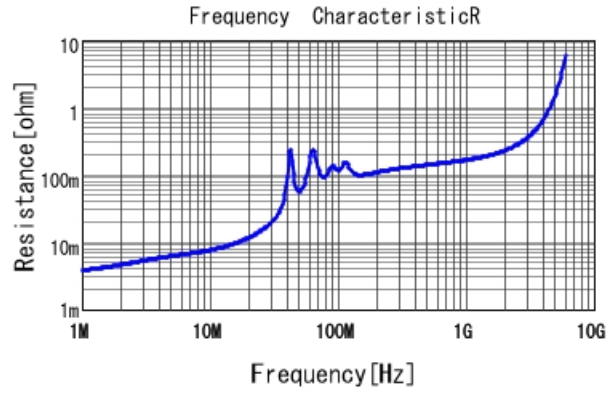
■ GRM31C5C1H563JA01 R DCOV, 25degC
