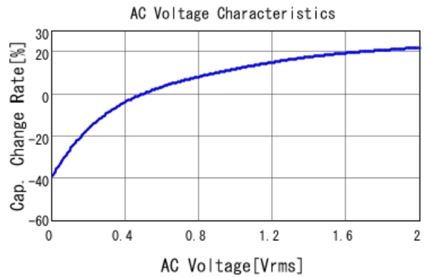
■ GCJ32ER70J476KE01 C-AC Voltage capchange, DC0V, 25.0d
