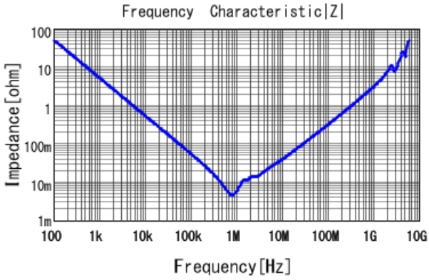
■ GCJ32ER70J476KE01 |Z| DC0V, 25degC
