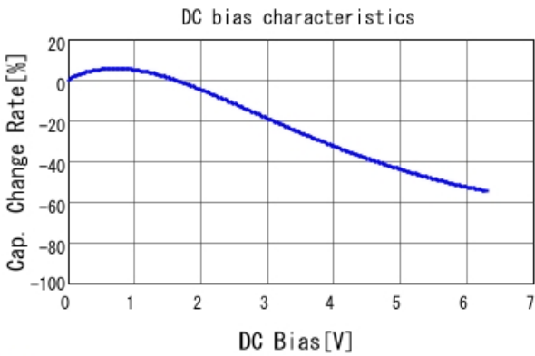
■ GCJ32ER70J476KE01 C-DC bias capchange, 25.0degC, AC0.
