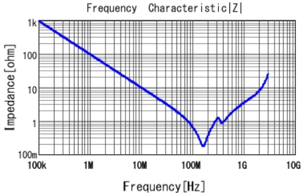
■ GA355QR7GF182KW01 |Z| DC0V, 25degC
