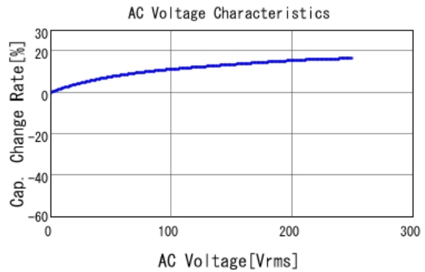
■ GA355QR7GF182KW01 C-AC Voltage capchange, DC0V, 25.0d
