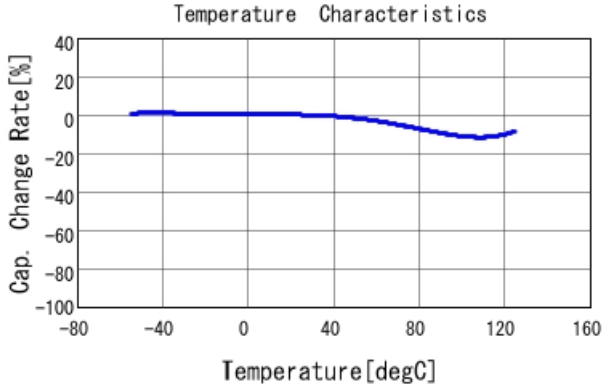
■ GA355QR7GF182KW01 C-Temp. capchange, DCOV, AC1Vrms
