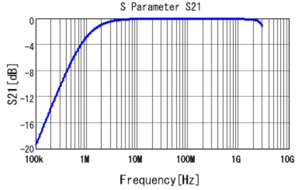
■ GA355QR7GF182KW01 S21 DCOV, 25degC
