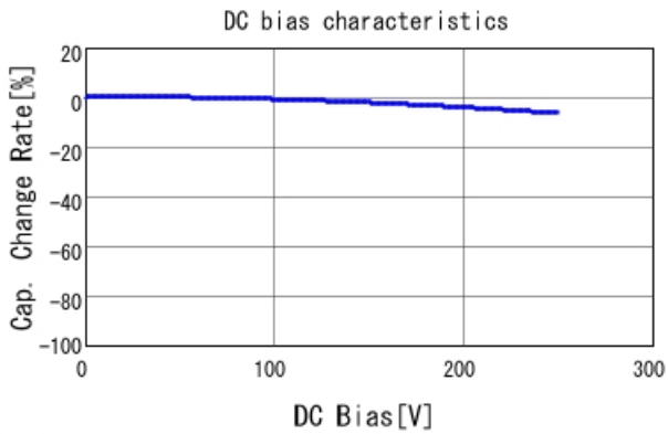
■ GA355QR7GF182KW01 C-DC bias capchange, 25.0degC, AC1V
