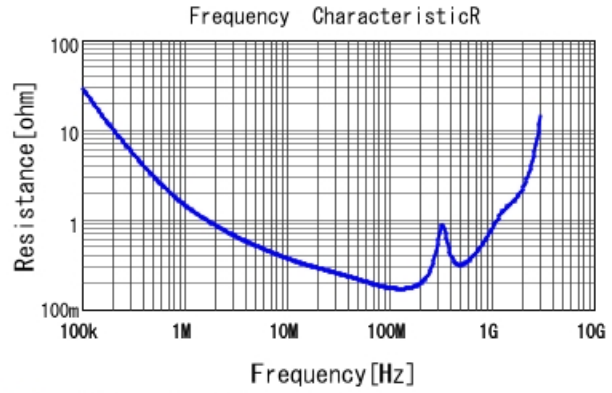
■ GA355QR7GF182KW01 R DC0V, 25degC
