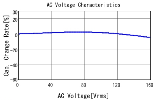
■ GC332DD72W104KX01 C-AC Voltage capchange, DC0V, 25.0d
