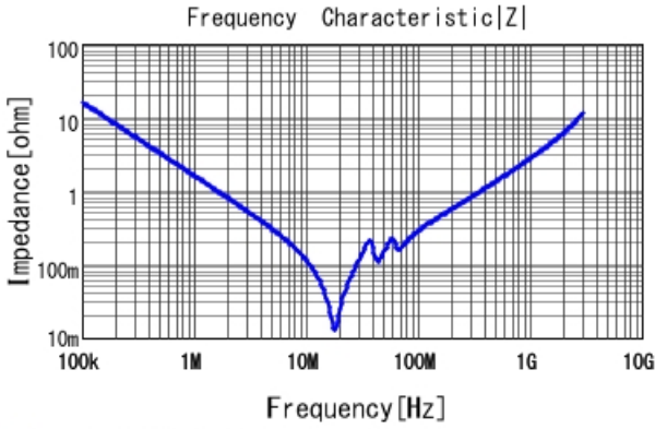
■ GC332DD72W104KX01 |Z| DC0V, 25degC
