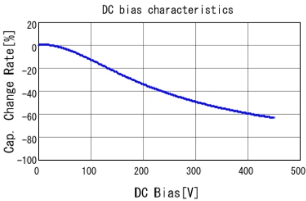
■ GC332DD72W104KX01 C-DC bias capchange, 25.0degC, AC1V
