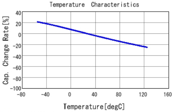
■ GC332DD72W104KX01 C-Temp. capchange, DCOV, AC1Vrms
