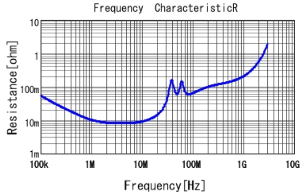
■ GC332DD72W104KX01 R DC0V, 25degC
