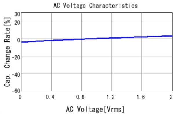
GCD188R71E333KA01 C-AC Voltage capchange, DC0V, 25.0d
