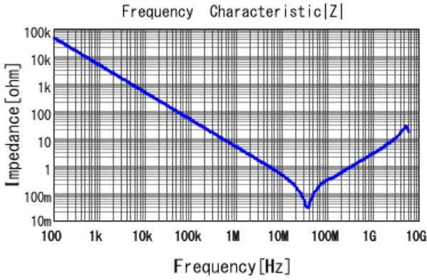
GCD188R71E333KA01 |Z| DC0V, 25degC
