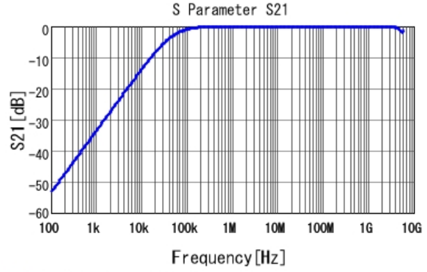
■ GCD188R71E333KA01 S21 DCOV, 25degC
