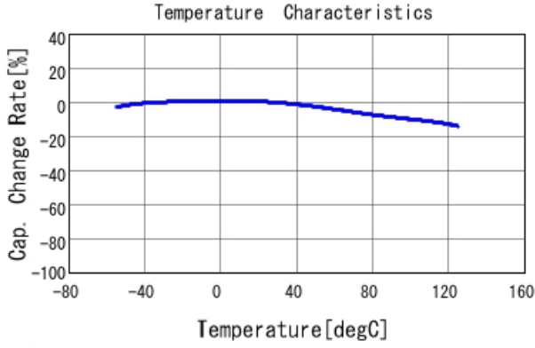
■ GCD188R71E333KA01 C-Temp. capchange, DCO. 0V, AC1.0V rm
