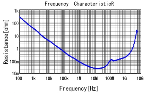
GCD188R71E333KA01 R DC0V, 25degC
