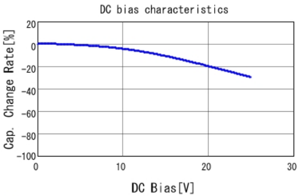
GCD188R71E333KA01 C-DC bias capchange, 25.0degC, AC1.
