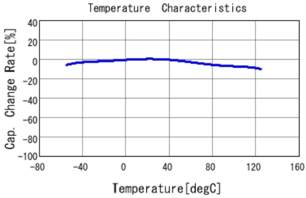
■ GCD21BR72A333KA01 C-Temp. capchange, DCO. 0V, AC1. 0Vrm
