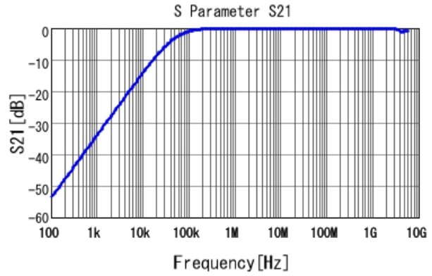
■ GCD21BR72A333KA01 S21 DCOV, 25degC
