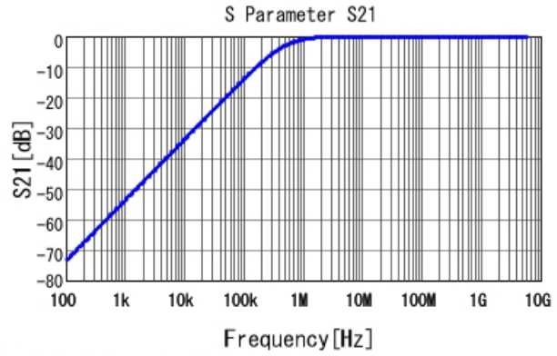
■ GCE188R72A332KA01 S21 DCOV, 25degC
