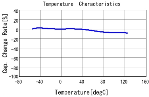
■ GCE188R72A332KA01 C-Temp. capchange, DCO. 0V, AC1. 0Vrm
