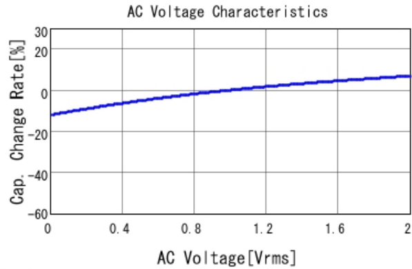
■ GCJ188R91H104KA01 C-AC Voltage capchange, DC0V, 25.0d
