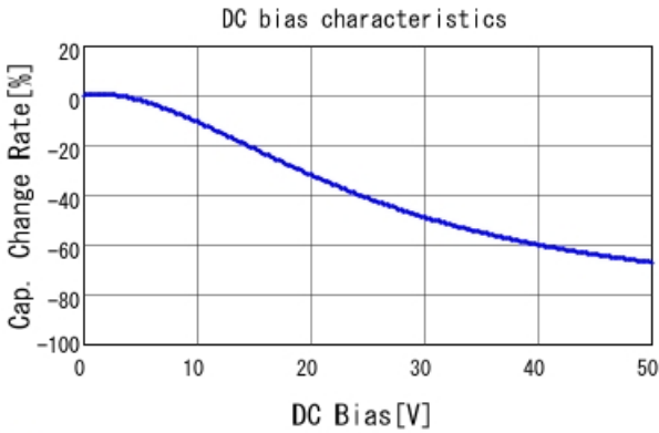
■ GCJ188R91H104KA01 C-DC bias capchange, 25.0degC, AC1.
