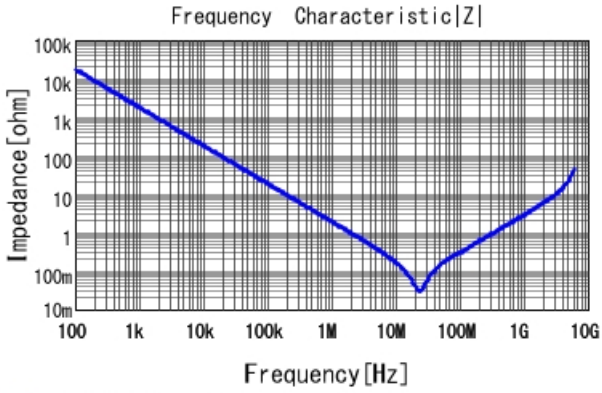
■ GCJ188R91H104KA01 |Z| DC0V, 25degC
