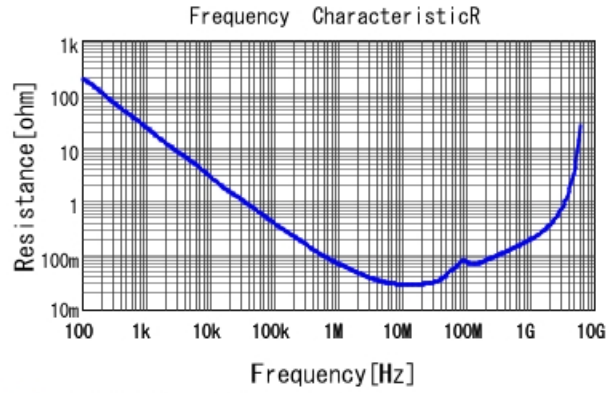
■ GCJ188R91H104KA01 R DC0V, 25degC
