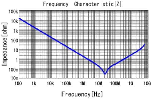
■ GCJ188R91H124KA01 |Z| DCOV, 25degC
