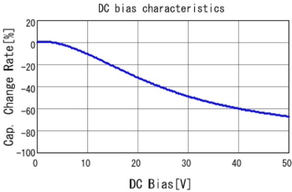
■ GCJ188R91H124KA01 C-DC bias capchange, 25.0degC, AC1.
