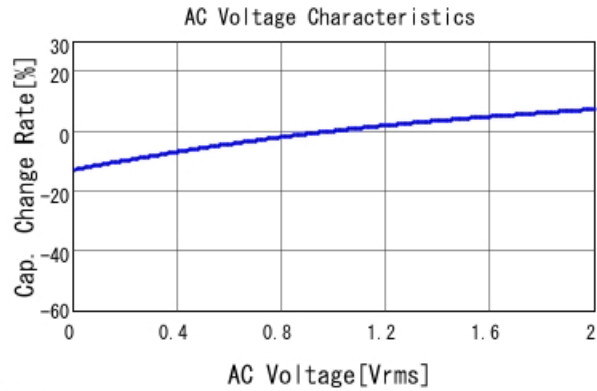
■ GCJ188R91H124KA01 C-AC Voltage capchange, DCOV, 25.0d
