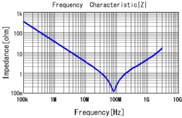
■ GCJ31BR72J472KXJ1 |Z| DC0V, 25degC
