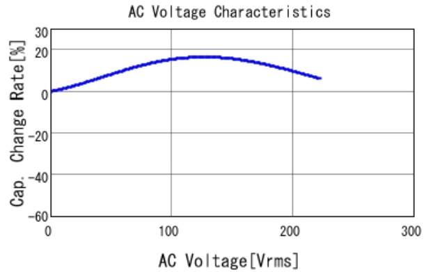
■ GCJ31BR72J472KXJ1 C-AC Voltage capchange, DC0V, 25.0d
