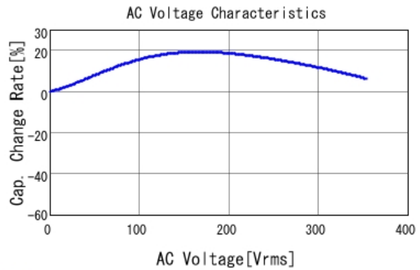
■ GCJ31BR73A152KXJ1 C-AC Voltage capchange, DC0V, 25.0d
