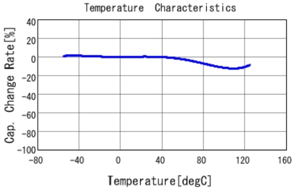
■ GCJ31BR73A152KXJ1 C-Temp. capchange, DCOV, AC1Vrms
