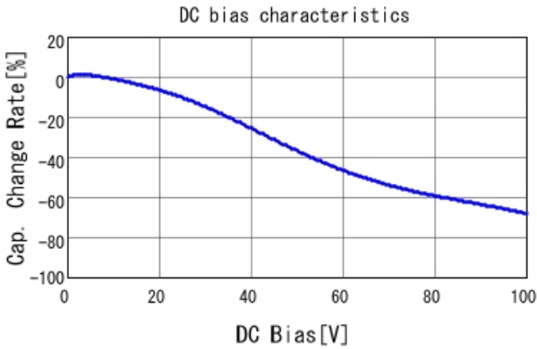
■ GCJ31MR72A154KA01 C-DC bias capchange, 25.0degC, AC1.
