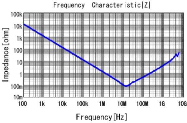
■ GCJ31MR72A154KA01 |Z| DCOV, 25degC
