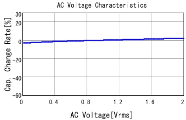
■ GCJ31MR72A154KA01 C-AC Voltage capchange, DCOV, 25.0d
