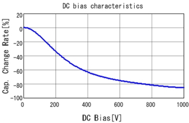
■ GCJ43DR73A333KXJ1 C-DC bias capchange, 25.0degC, AC1V
