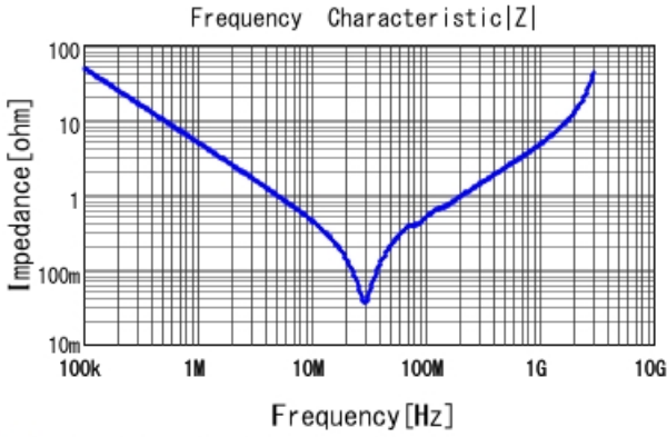
■ GCJ43DR73A333KXJ1 |Z| DC0V, 25degC
