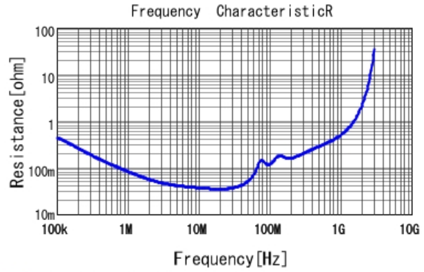
■ GCJ43DR73A333KXJ1 R DC0V, 25degC
