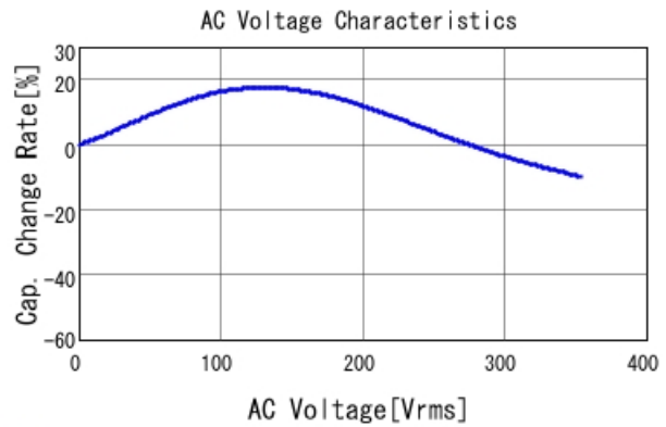
■ GCJ43DR73A333KXJ1 C-AC Voltage capchange, DC0V, 25.0d
