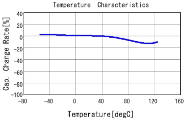
■ GCJ43DR73A333KXJ1 C-Temp. capchange, DCOV, AC1Vrms
