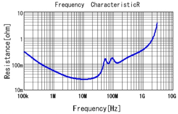
■ GCJ43DR73A473KXJ1 R DC0V, 25degC
