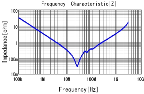
■ GCJ43DR73A473KXJ1 |Z| DC0V, 25degC
