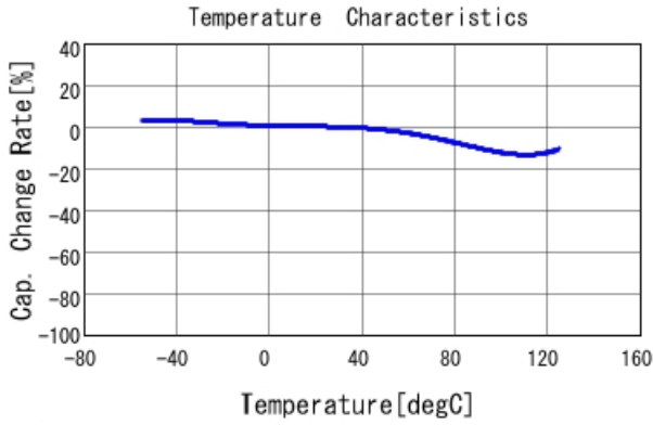
■ GCJ43DR73A473KXJ1 C-Temp. capchange, DCOV, AC1Vrms
