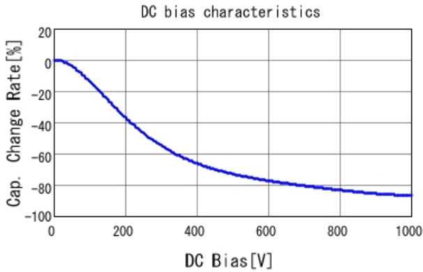
■ GCJ43DR73A473KXJ1 C-DC bias capchange, 25.0degC, AC1V
