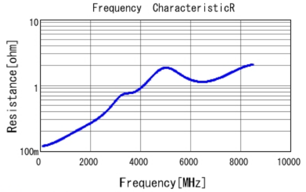
GCM0335C1H510JA16 R DCOV, 25degC
