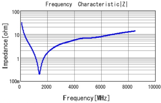
GCM0335C1H510JA16 |Z| DCOV, 25degC
