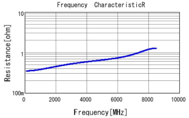
■ GCM1555C1H1R8WA16 R DCOV, 25degC
