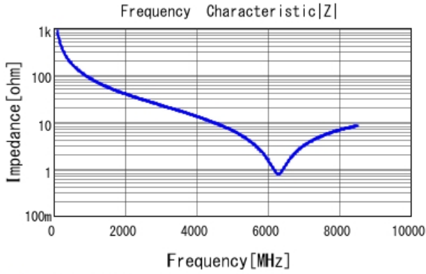
■ GCM1555C1H1R8WA16 |Z| DCOV, 25degC
