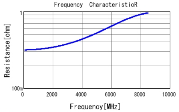
GCM1555C1H2R2BA16 R DC0V, 25degC
