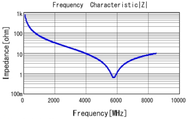
GCM1555C1H2R2BA16 |Z| DC0V, 25degC
