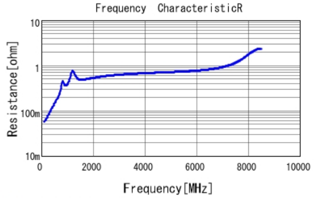
■ GCM1555C1H471JA16 R DCOV, 25degC
