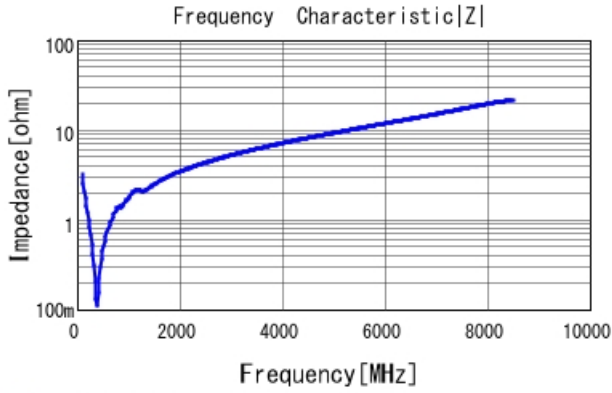
■ GCM1555C1H471JA16 |Z| DCOV, 25degC
