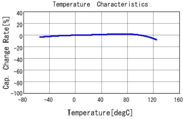
GCM155R71C154KE02 C-Temp. capchange, DCO. 0V, AC1. 0Vrm
