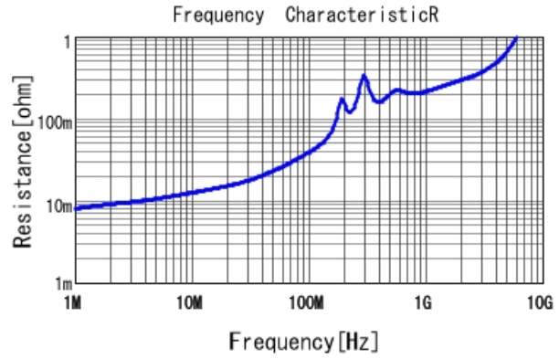
GCM1885C1H622JA16 R DCOV, 25degC
