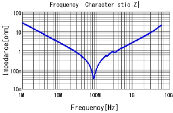
GCM1885C1H622JA16 |Z| DCOV, 25degC
