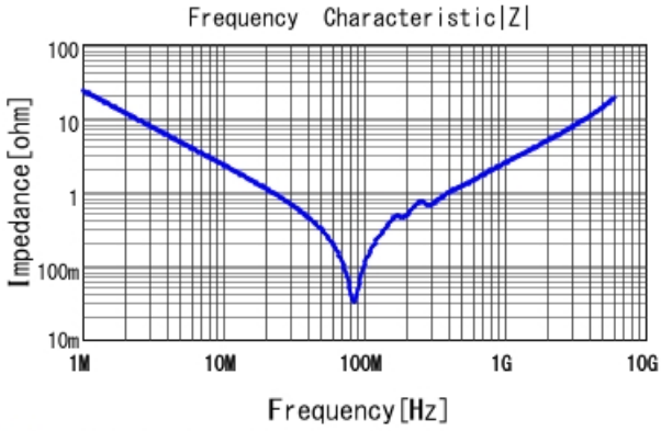
GCM1885C1H682JA16 |Z| DCOV, 25degC
