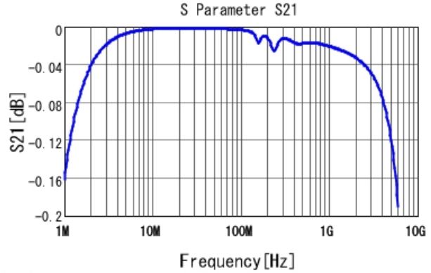
■ GCM1885C1H822JA16 S21 DCOV, 25degC
