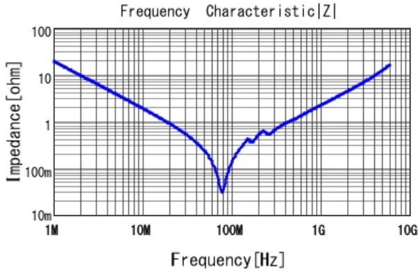
GCM1885C1H822JA16 |Z| DCOV, 25degC
