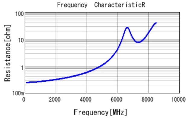
GCM1885C2A5R0BA16 R DCOV, 25degC
