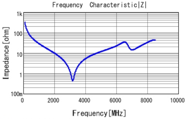
GCM1885C2A5R0BA16 |Z| DCOV, 25degC
