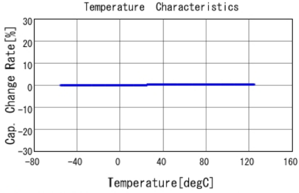
■ GCM1885C2A5R0BA16 C-Temp. capchange, DCOV, AC1Vrms
