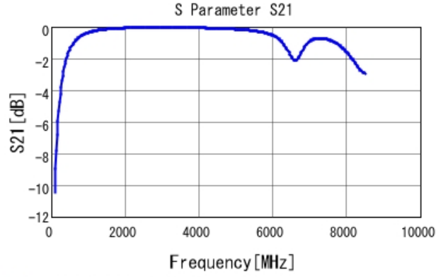
■ GCM1885C2A5R0BA16 S21 DCOV, 25degC
