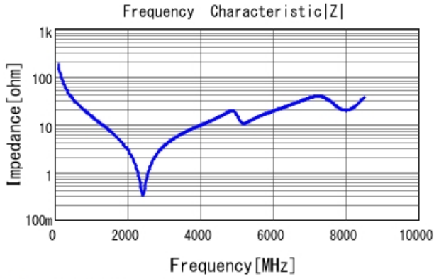
■ GCM1885C2A9R0BA16 |Z| DCOV, 25degC
