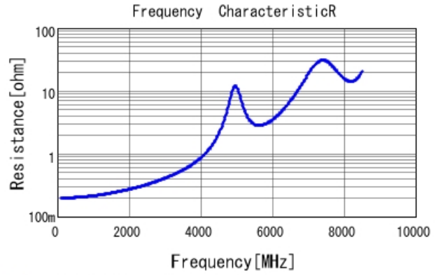
■ GCM1885C2A9R0BA16 R DCOV, 25degC
