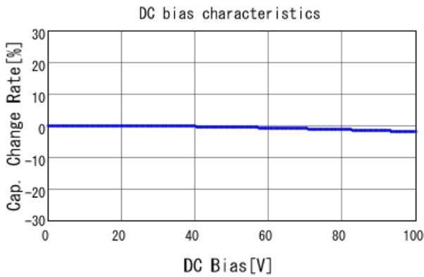
■ GCM1887U2A102JA16 C-DC bias capchange, 25.0degC, AC1V
