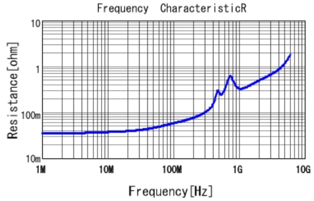
■ GCM1887U2A102JA16 R DCOV, 25degC
