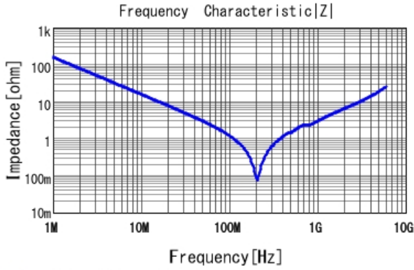
■ GCM1887U2A102JA16 |Z| DCOV, 25degC
