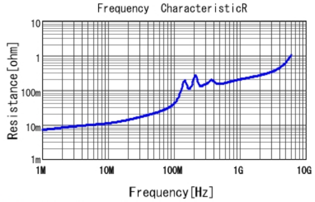
■ GCM1887U2A103JA16 R DCOV, 25degC
