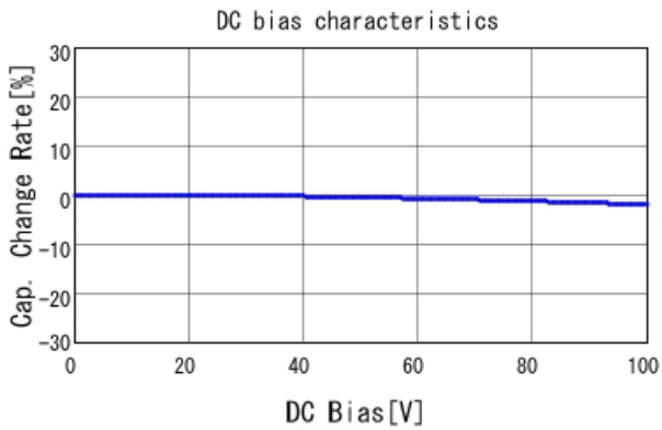
■ GCM1887U2A103JA16 C-DC bias capchange, 25.0degC, AC1V
