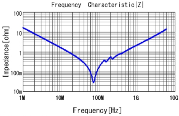
■ GCM1887U2A103JA16 |Z| DCOV, 25degC
