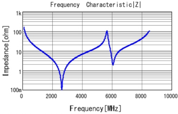
■ GQM1875G2E100JB12 |Z| DC0V, 25degC
