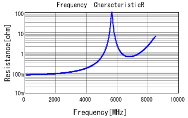
■ GQM1875G2E100JB12 R DC0V, 25degC
