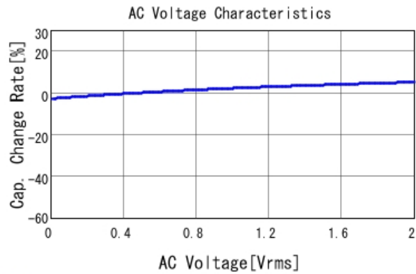
■ GRJ32EC71E226KE11 C-AC Voltage capchange, DC0V, 25.0d
