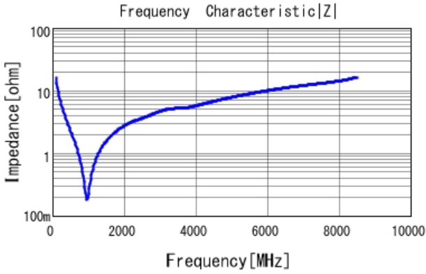
■ GRM0335C1E101JA01 |Z| DCOV, 25degC
