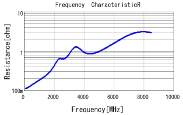
■ GRM0335C1E101JA01 R DCOV, 25degC
