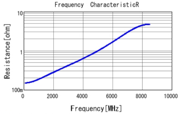
■ GRM0335C1E270JA01 R DCOV, 25degC
