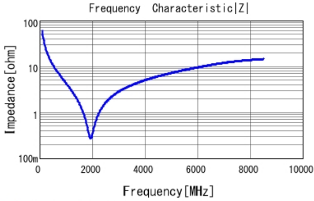
■ GRM0335C1E270JA01 |Z| DCOV, 25degC
