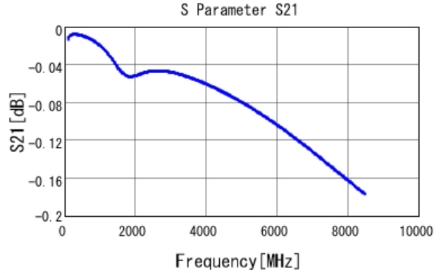
■ GRM0335C1E391JA01 S21 DCOV, 25degC
