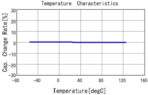
■ GRM0335C1E391JA01 C-Temp. capchange, DCOV, AC1Vrms
