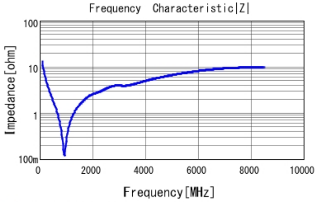
■ GRM0335C1H121JA01 |Z| DCOV, 25degC
