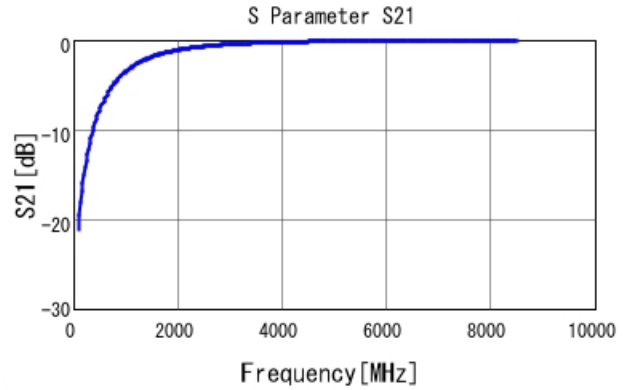
■ GRM0335C2A1R4WA01 S21 DCOV, 25degC
