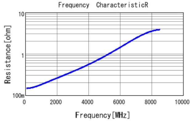
■ GRM0335C2A330JA01 R DC0V, 25degC
