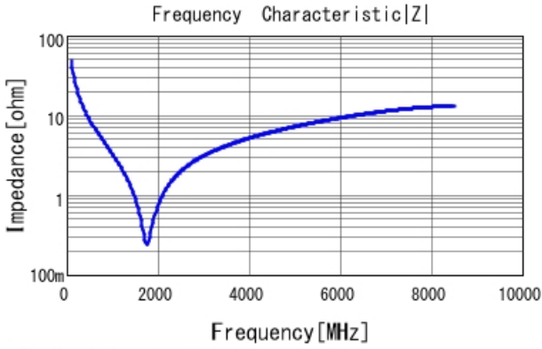
■ GRM0335C2A330JA01 |Z| DC0V, 25degC
