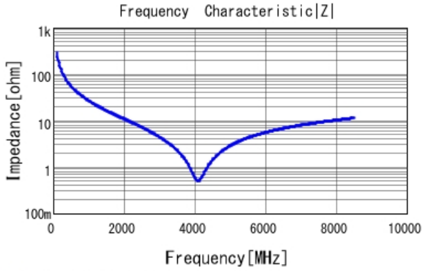
■ GRM0335C2A5R6WA01 |Z| DCOV, 25degC
