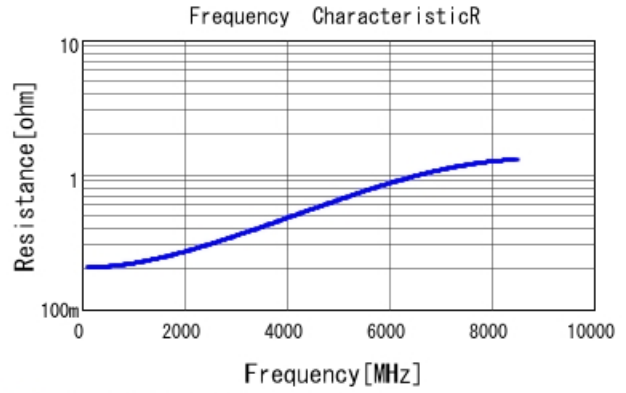
■ GRM0335C2A5R6WA01 R DCOV, 25degC
