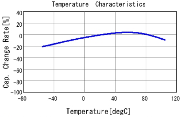
■ GRM155C81C105KE11 C-Temp. capchange, DCO. 0V, ACO. 2Vrm
